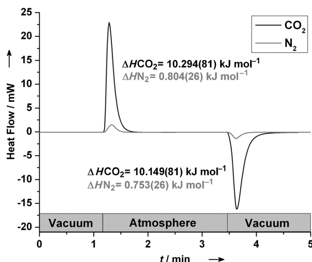
Figure 3. Vacuum swing adsorption DSC data for one cycle of CO 2 and N 2 loading/unloading in the CaSDB framework.
